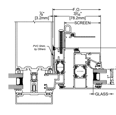
3B JAMB CURTAIN WALL INSTALLATION
