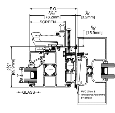
4A JAMB STOREFRONT INSTALLATION
