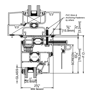
1A HEAD STOREFRONT INSTALLATION
