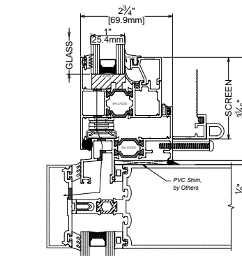
2B SILL CURTAIN WALL INSTALLATION
