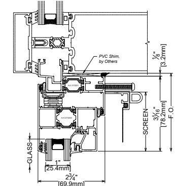
1B HEAD CURTAIN WALL INSTALLATION
