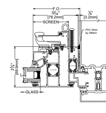
4B JAMB CURTAIN WALL INSTALLATION
