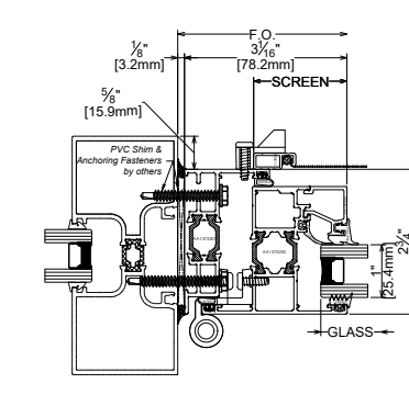
7A JAMB STOREFRONT INSTALLATION
