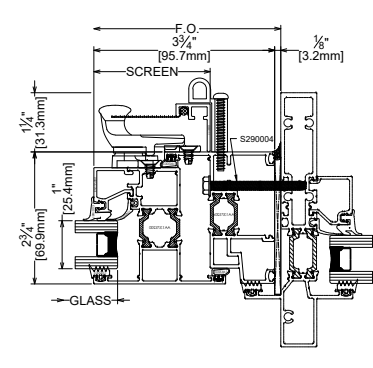
4 JAMB EQUAL LEG INSTALLATION
