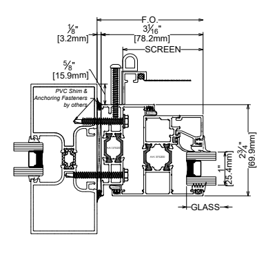
3A JAMB STOREFRONT INSTALLATION
