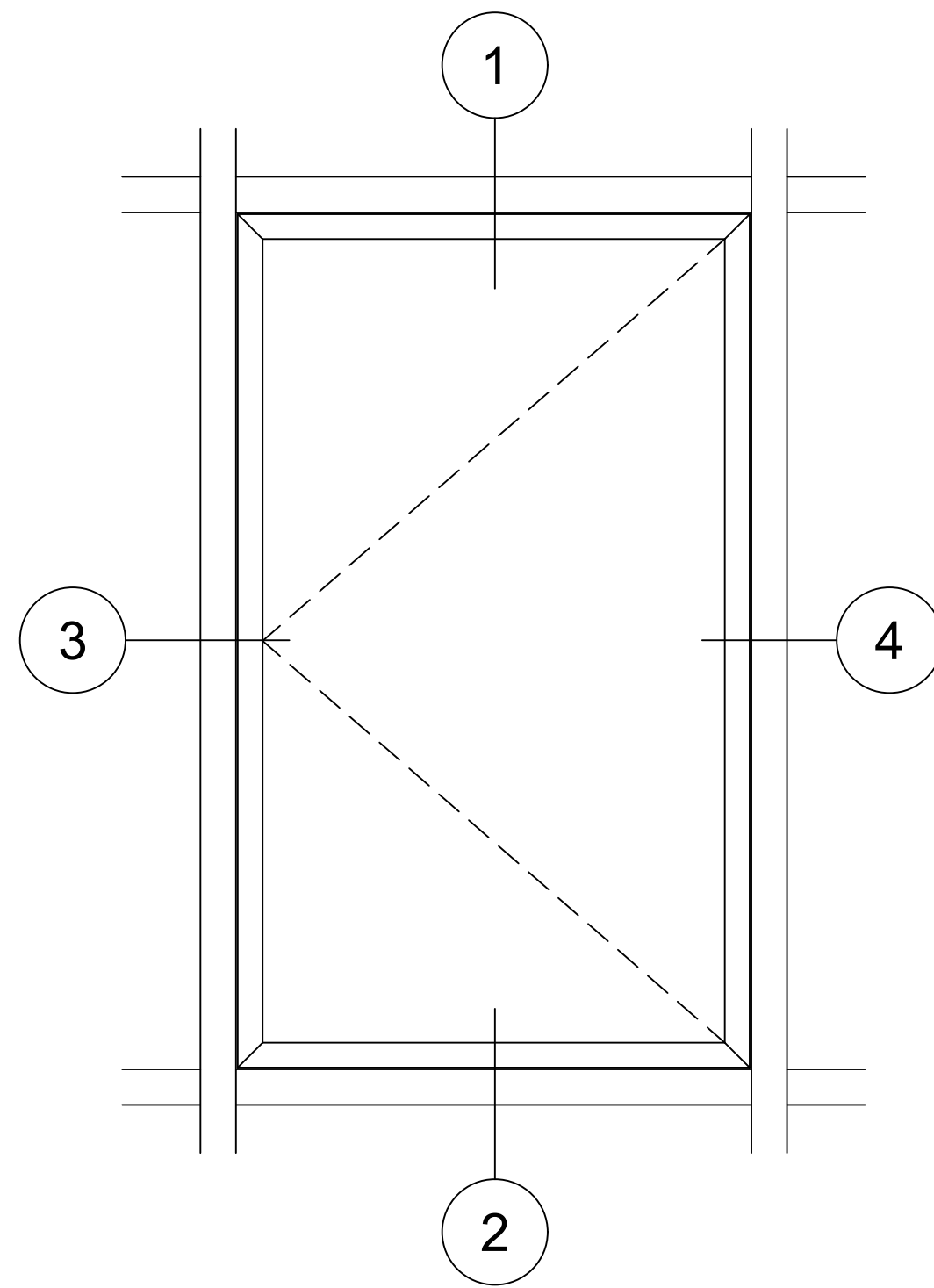
TYPICAL ELEVATION 4-BAR / MPL WITH OPTIONAL SCREEN
