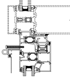
Curtain Wall Integration
