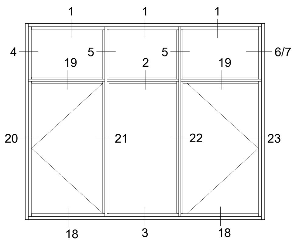
TYPICAL ELEVATION 2970AW SHADOWLINE WITH TRIPLE GLAZED
