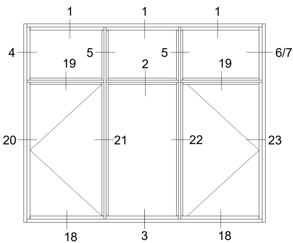
TYPICAL ELEVATION 2970AW SHADOWLINE
