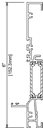
Sill Frame Tpl. Glazed
