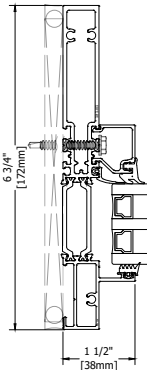
MITERED FRAME ASSEMBLY ∠ 45°
