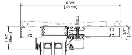
1 MITERED FRAME ASSEMBLY ∠ 45°
