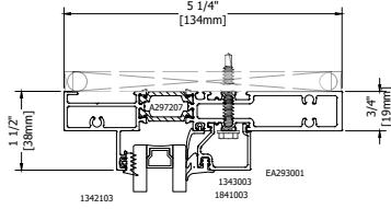
1 MITERED FRAME ASSEMBLY ∠ 45°
