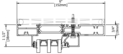
1 MITERED FRAME ASSEMBLY ∠ 45°
