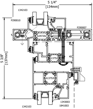
5 1/4" Deep w/ 1375 1375 PO Casement
