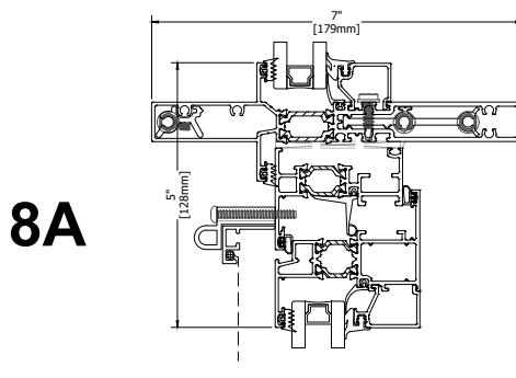
7.00" Deep w/ 1375 PI Casement
