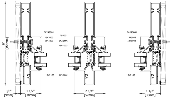
MITERED FRAME ASSEMBLY ∠ 45°
