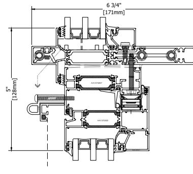
6.75" Deep w/ 1375 PI Casement
