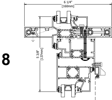
6" Deep w/ 1375 PO Casement
