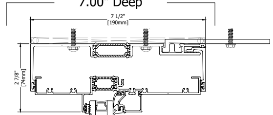
1A OPTIONAL w/ HEAD RECEPTOR
