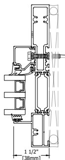
MITERED FRAME ASSEMBLY ∠ 45°
