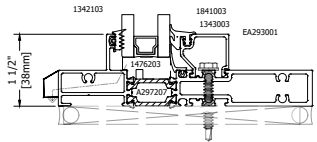
MITERED FRAME ASSEMBLY ∠ 45°
