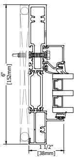
MITERED FRAME ASSEMBLY ∠ 45°
