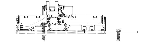
3A OPTIONAL SILL w/ SILL RECEPTOR
