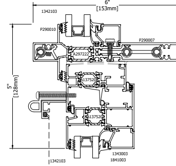
6.00" Deep w/ 1375 PI Casement
