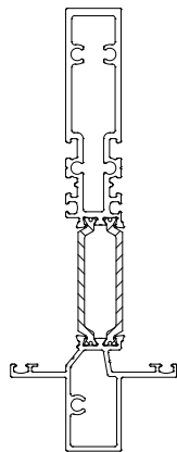
Intermediate Frame Tpl. Glazed
