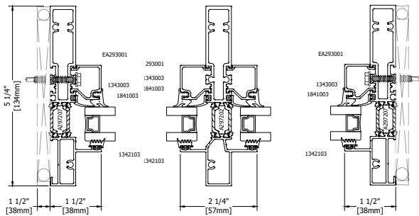
MITERED FRAME ASSEMBLY ∠ 45°
