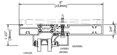
1 MITERED FRAME ASSEMBLY ∠ 45°
