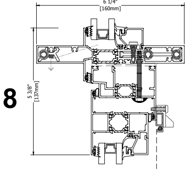
6 1/4" Deep w/ 1375 PO Awning
