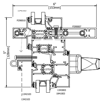
6.00" Deep w/ 1375 PI HOPPER
