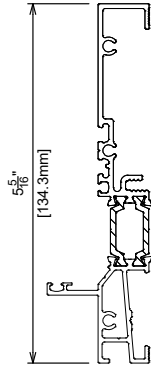
Sill Frame Dbl. Glazed
