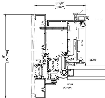
6.00" Deep w/ 5000 Phantom Vent Casement ROTO & MPL Handle
