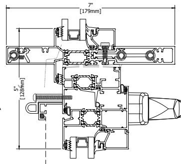
7.00" Deep w/ 1375 PI HOPPER
