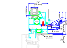
6B SEUIL INSERTION MUR-RIDEAU
