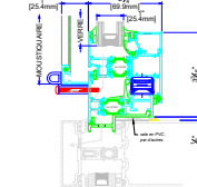
2B SEUIL INSERTION MUR-RIDEAU
