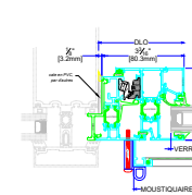
3B JAMBAGE INSERTION MUR-RIDEAU
