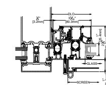
3B JAMB CAPTURED INSTALLATION
