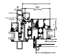
3 JAMB EQUAL LEG INSTALLATION
