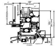
2 SILL EQUAL LEG INSTALLATION
