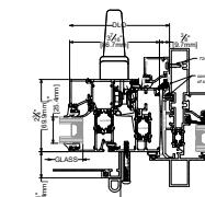
4 JAMB EQUAL LEG INSTALLATION
