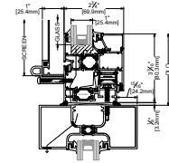
2A SILL FLATBACK INSTALLATION
