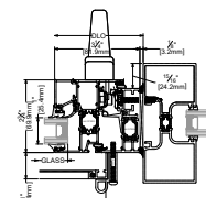
4A JAMB FLATBACK INSTALLATION
