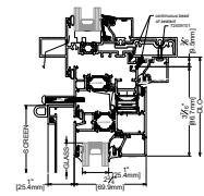
1 HEAD EQUAL LEG INSTALLATION
