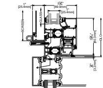
2B SILL CAPTURED INSTALLATION
