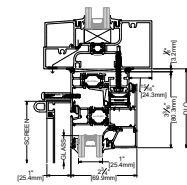
1A HEAD FLATBACK INSTALLATION
