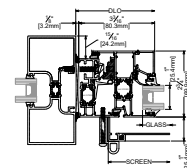
3A JAMB FLATBACK INSTALLATION
