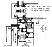
1B HEAD CAPTURED INSTALLATION
