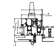
4B JAMB CAPTURED INSTALLATION
