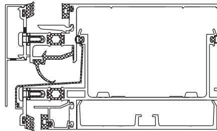
Double glazed capped system
