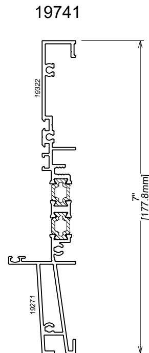
7" Rolled Sill Frame Tpl. Glazed
