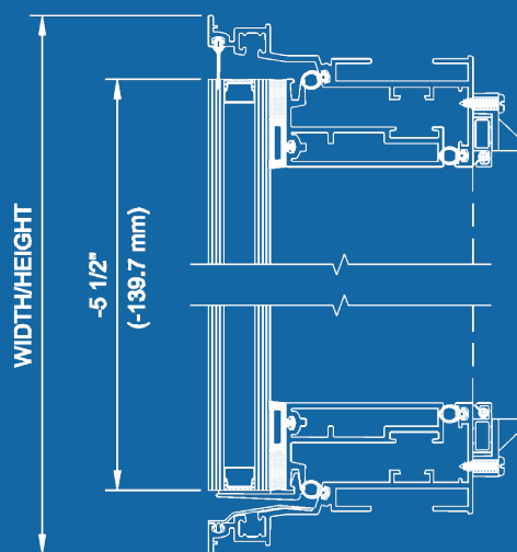
INSERT FOR CURTAIN WALL
