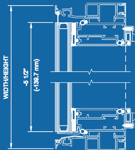
INSERT FOR FIXED WINDOW
